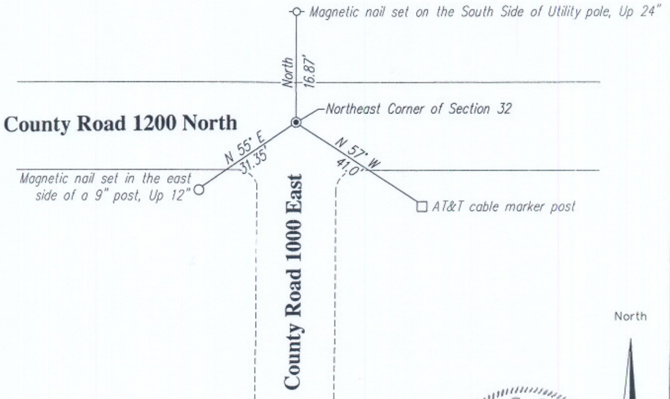
Reference Sketch
