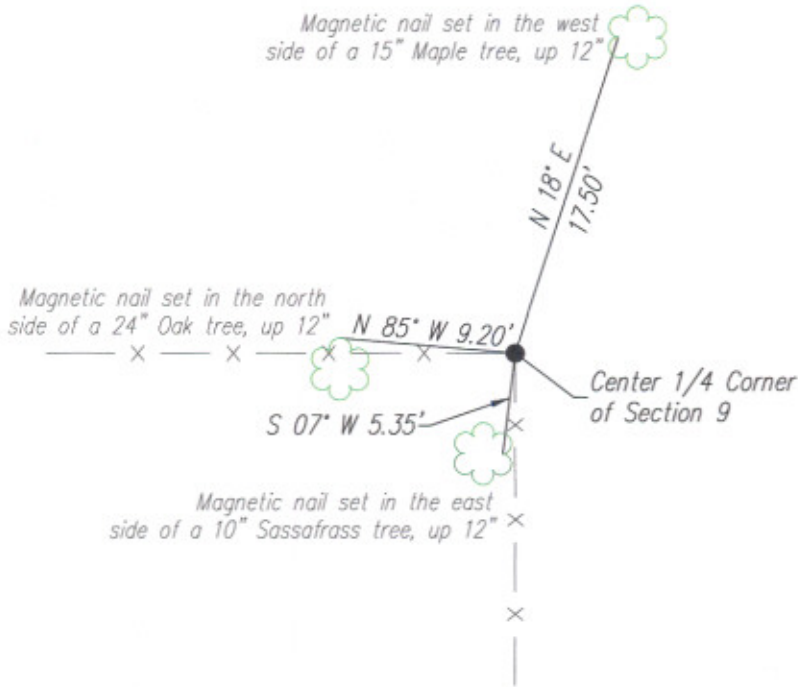
Reference Sketch
